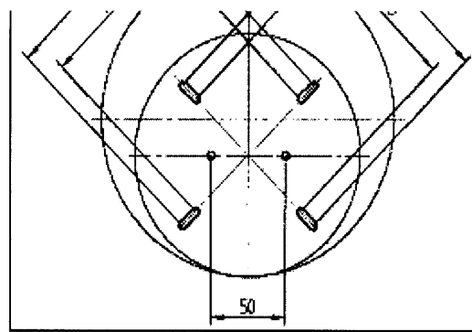
Fixing Details
