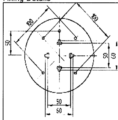
Fixing Details
