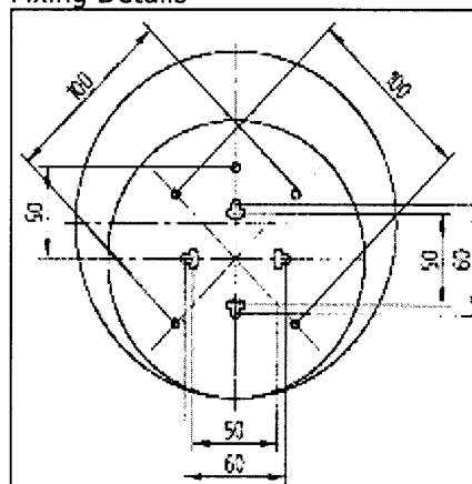
Fixing Details
