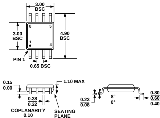
COMPLIANT TO JEDEC STANDARDS MO-187-AA Figure 33. 8-Lead Mini Small Outline Package [MINI_SO] (RM-8) Dimensions shown in millimeters
