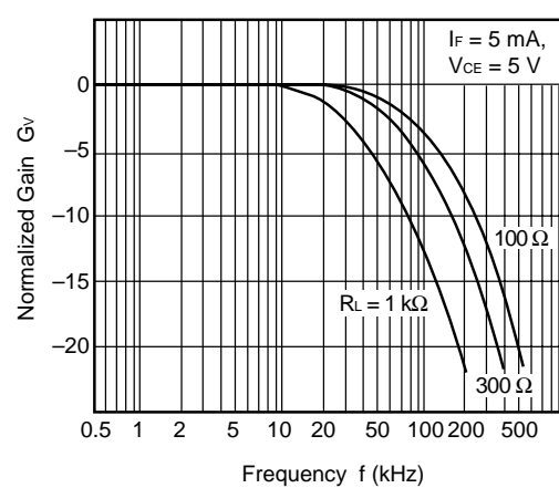
FREQUENCY RESPONSE
