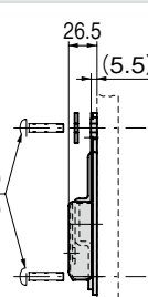
受け本体詳細 Catch body specifications
