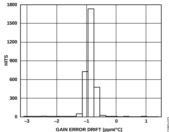
Figure 25. Gain Error Drift Distribution
