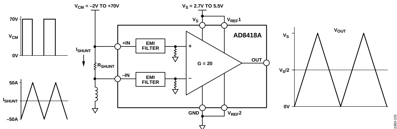
Figure 26. Typical Application
