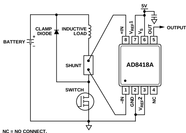
Figure 34. Low-Side Switch
