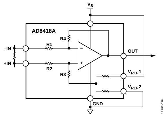
Figure 30. Split Supply
