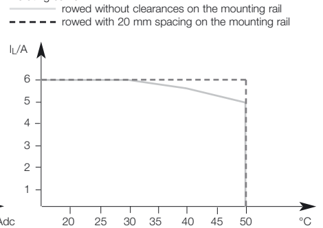
Derating curve
