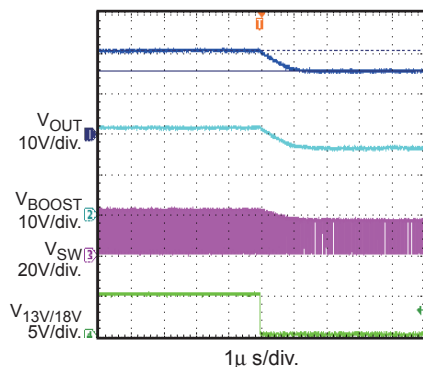
18V to 13V Switch
