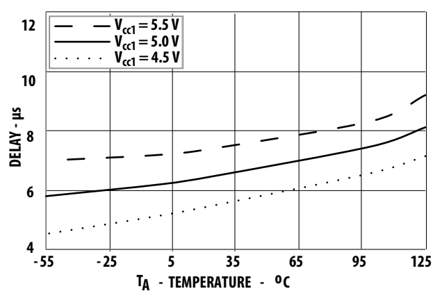
Figure 28 \overline{\text{RESET}} to High Level Fault Signal Delay vs. Temperature
