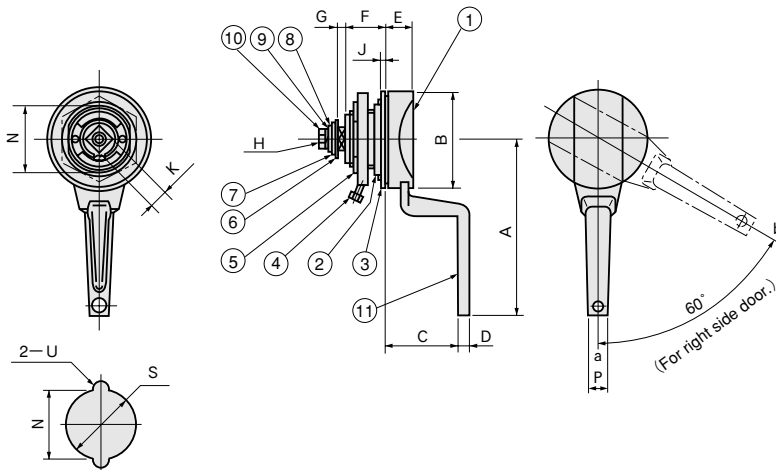
Layout of a Hole for Installation
