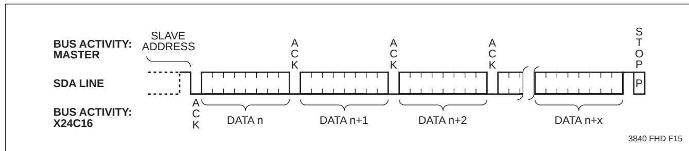
Figure 9. Sequential Read
