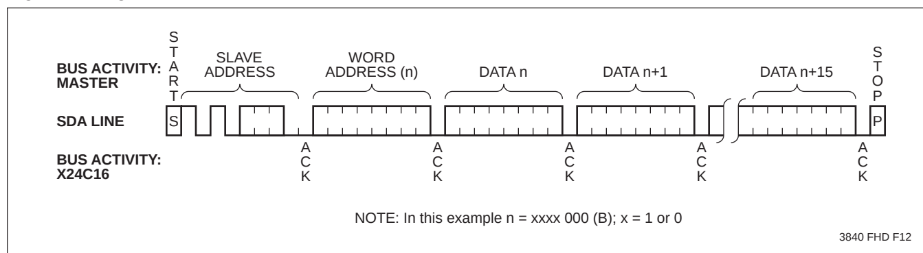
Figure 6. Page Write
