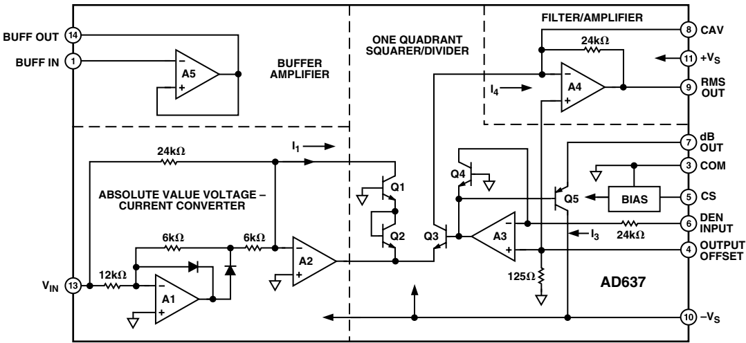
Figure 1. Simplified Schematic
