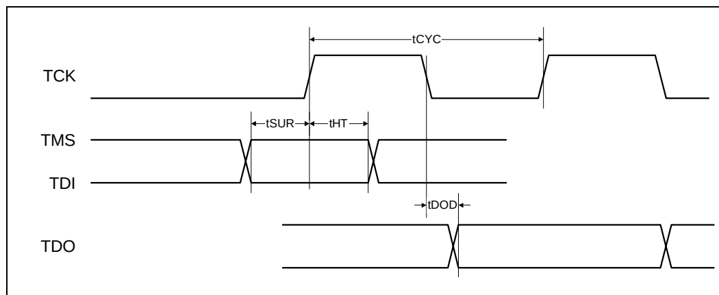
Figure 21. JTAG Timing
