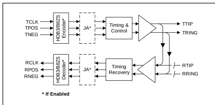
Figure 9. Analog Loopback
