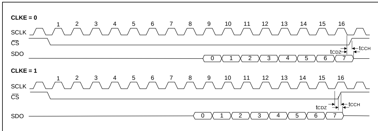
Figure 31. Serial Output Timing
