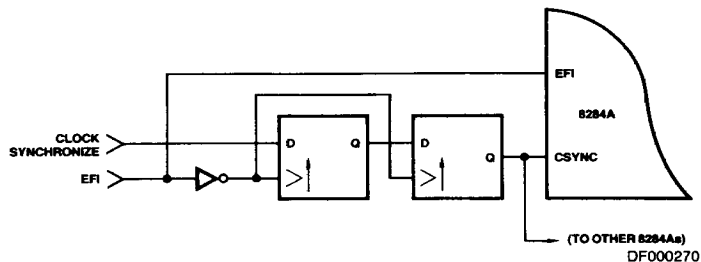
Figure 1. CSYNC Synchronization
