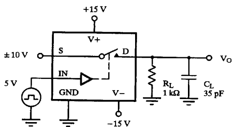
Figure 2. Switching Time
