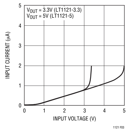
Figure 3. Input Current
