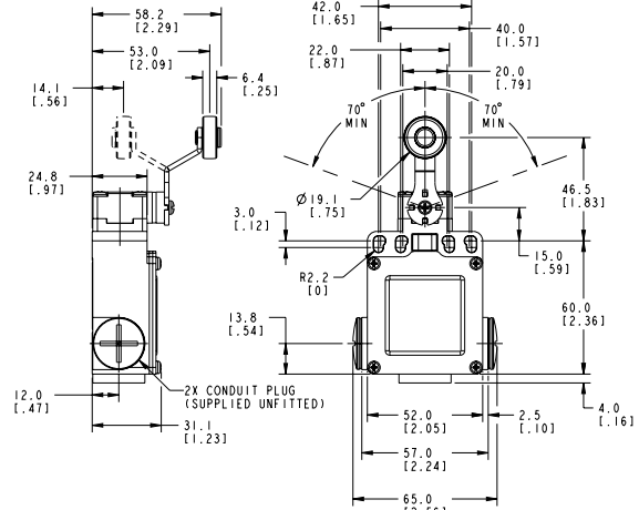
Figure 26. GLE Side Rotary • A5A and A5B
