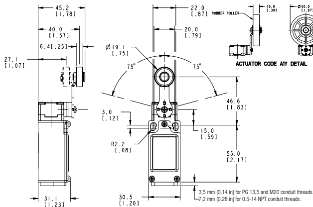
Figure 2. GLC Side Rotary • A2, A2A, A2B, and A2Y
