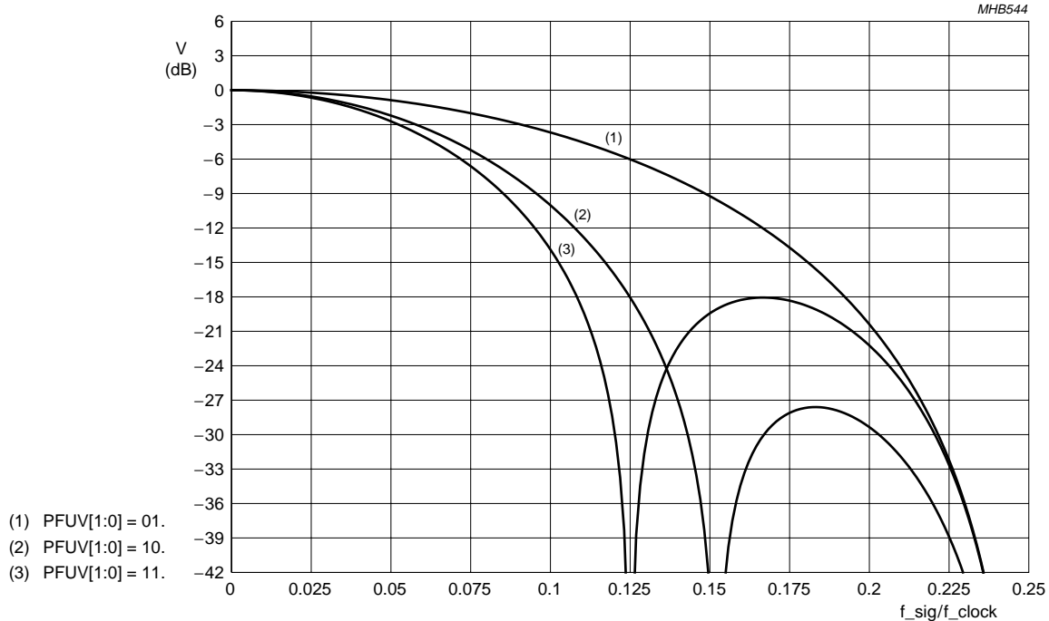
Fig.25 Chrominance prefilter characteristic.
