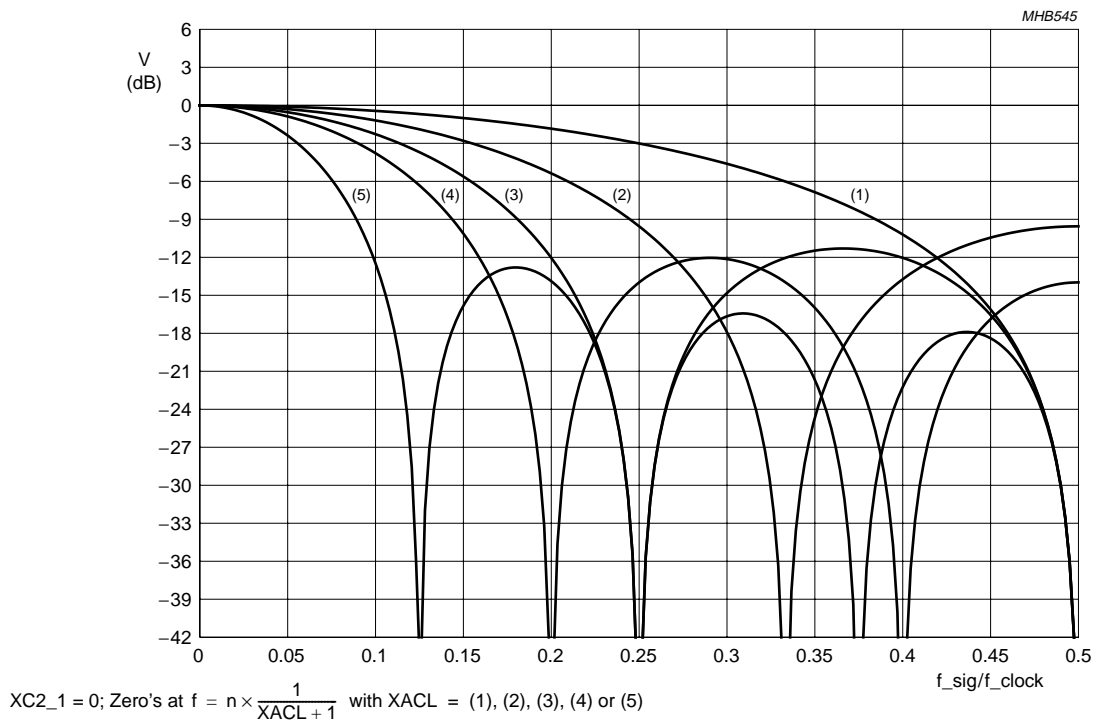
Fig.26 Examples for prescaler filter characteristics: effect of increasing XACL[5:0].
