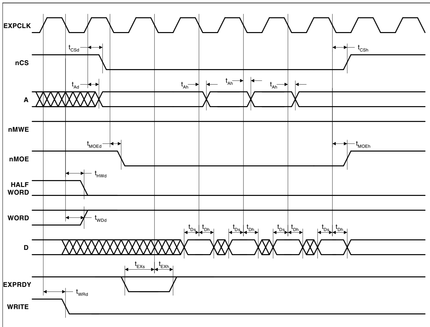
Figure 4. Static Memory Burst Read Cycle Timing Measurement
