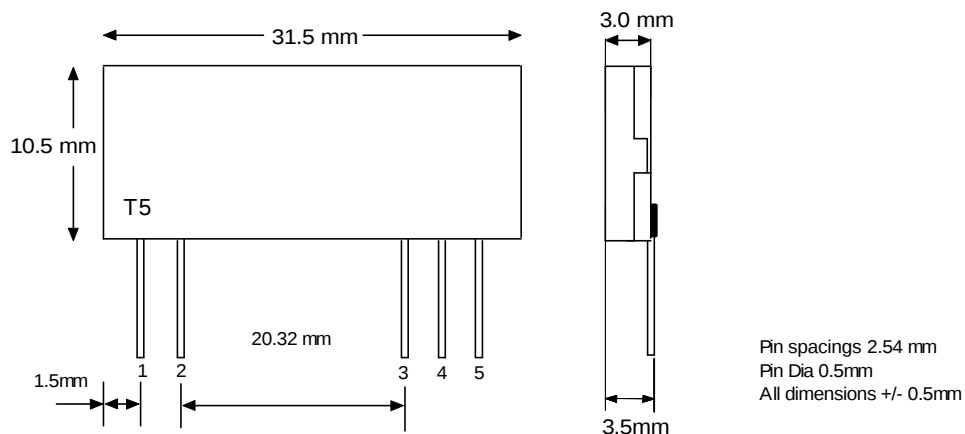
Figure 6: Transmitter
