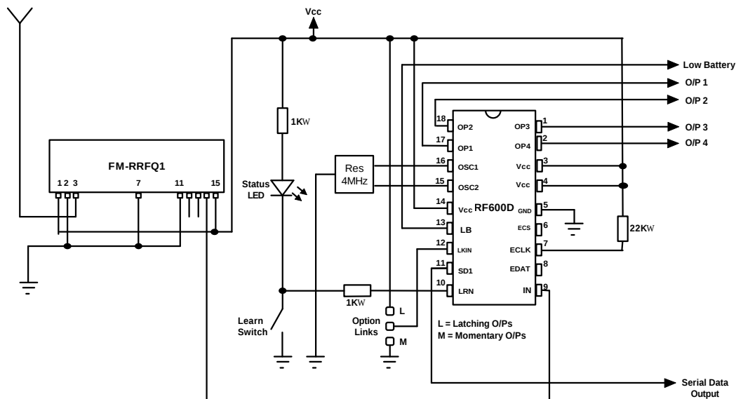
Receiver Circuit
