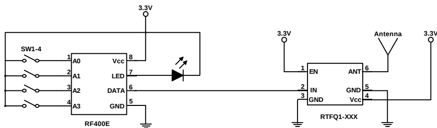
Transmitter Circuit
