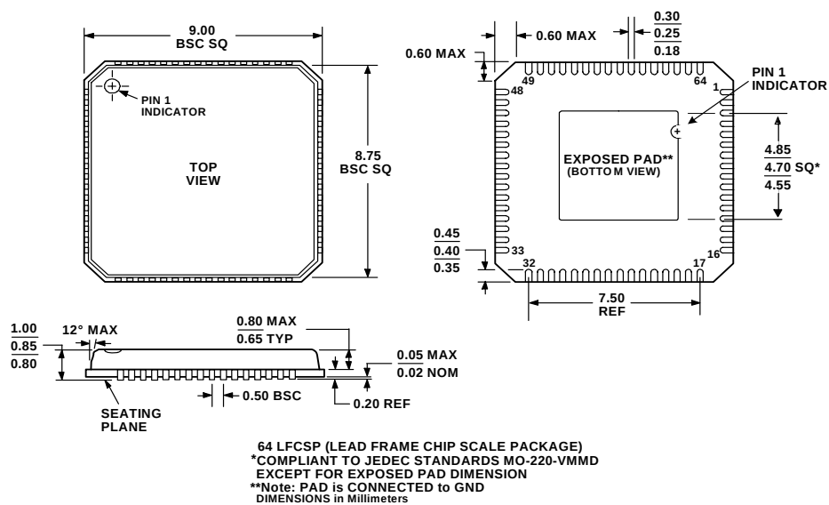
Figure 5. 64-Lead Lead Frame Chip Scale Package [LFCSP_VQ] 9 mm × 9 mm Body, Very Thin Quad (CP-64-1)
