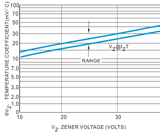
FIGURE 2 - TEMPERATURE COEFFICIENTS
