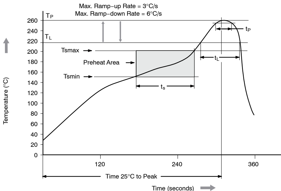
Figure 16. Reflow Profile
