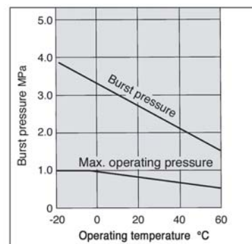
Burst Pressure Characteristics and Operating Pressure Curve
