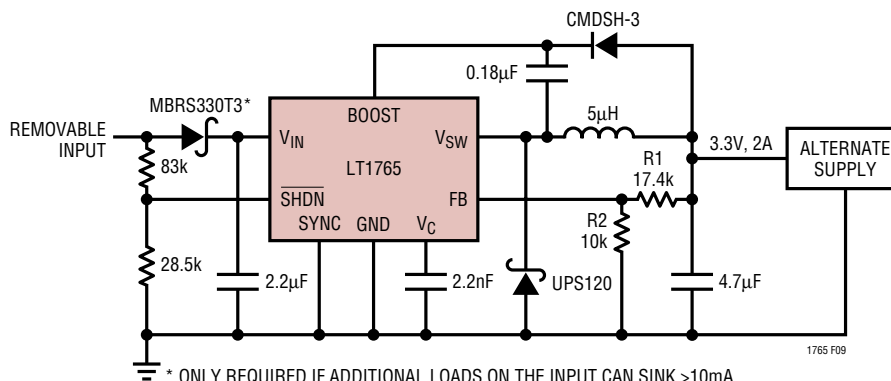
Figure 9. Dual Source Supply with 6µA Reverse Leakage
