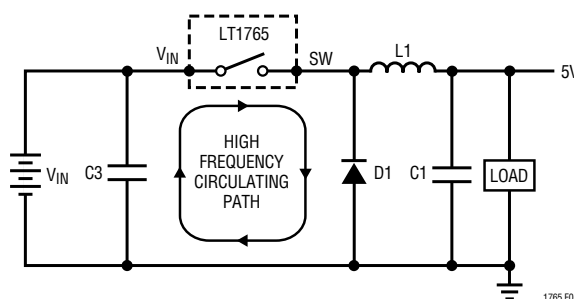
Figure 5. High Speed Switching Path
