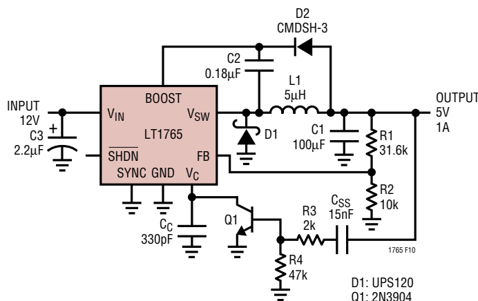
Figure 10. Buck Converter with Adjustable Soft Start
