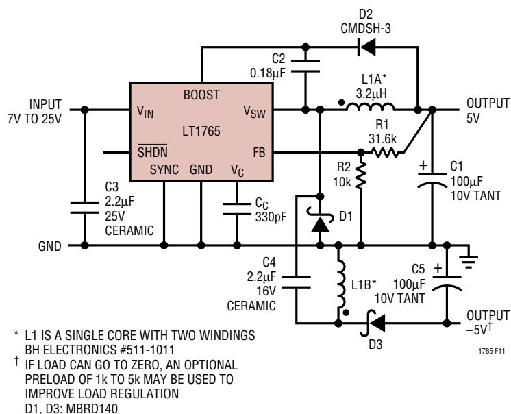
Figure 11. Dual Output Converter
