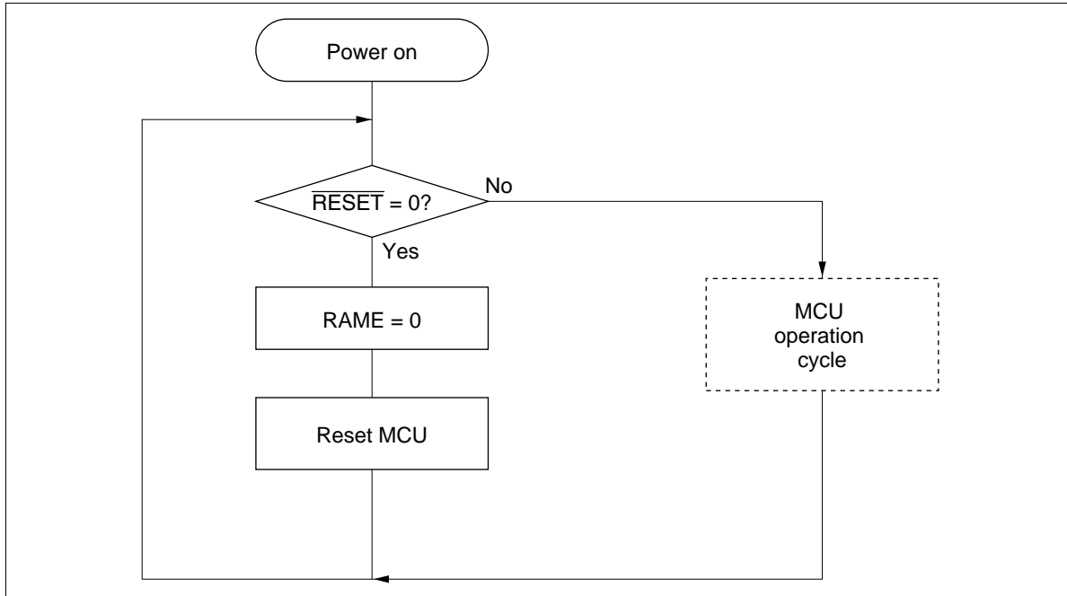
Figure 14 MCU Operating Sequence (power on)
