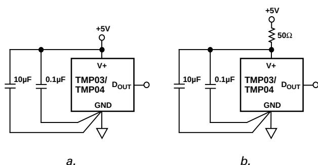
Figure 28. Recommended Supply Bypassing for the TMP03/TMP04
