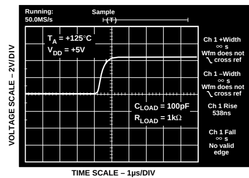
Figure 8. TMP03 Output Rise Time at +125°C
