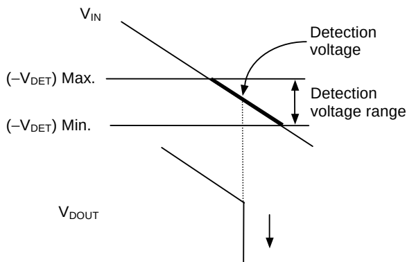
Figure 29 Detection Voltage
