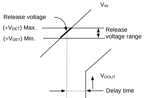
Figure 30 Release Voltage
