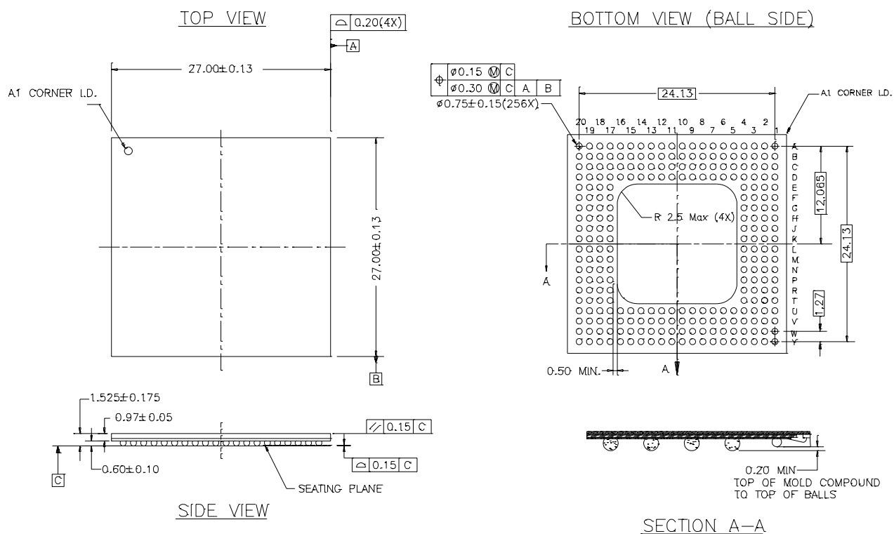
256-Lead Thermally Enhanced L2BGA (27 x 27 x 1.52 mm) BL256
