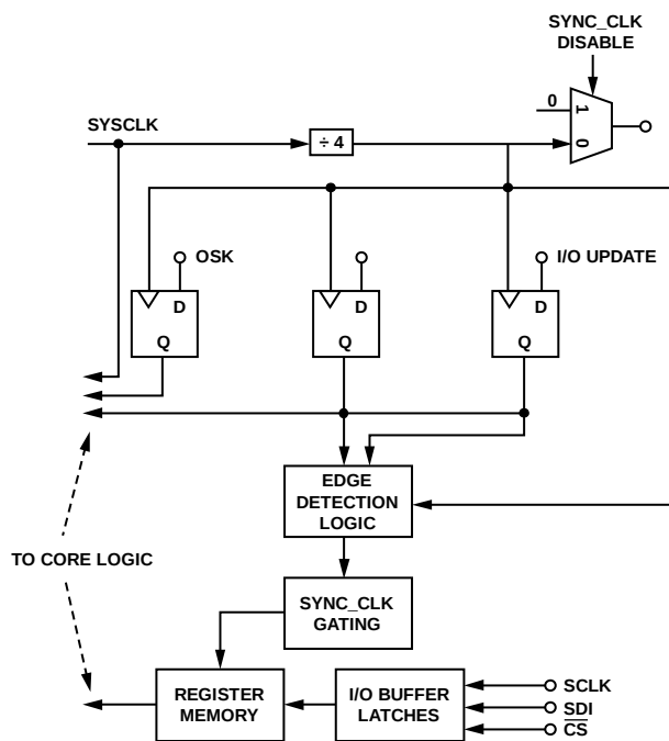
Figure 19. I/O Synchronization Block Diagram
