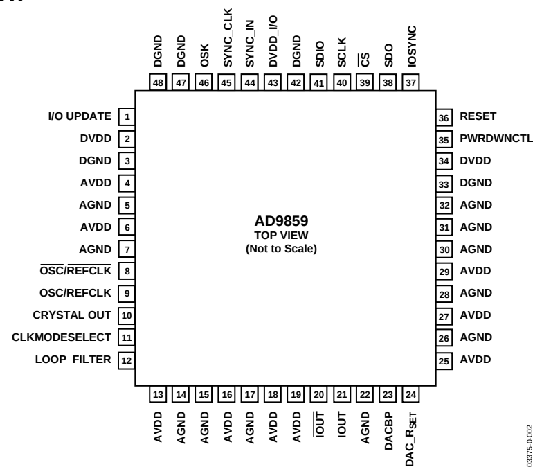
Figure 3. 48-Lead TQFP/EP
