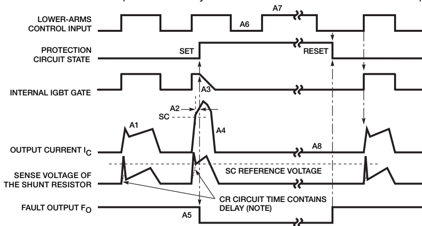
Short-Circuit Protection (Lower-arms only with the external shunt resistor and RC filter)
