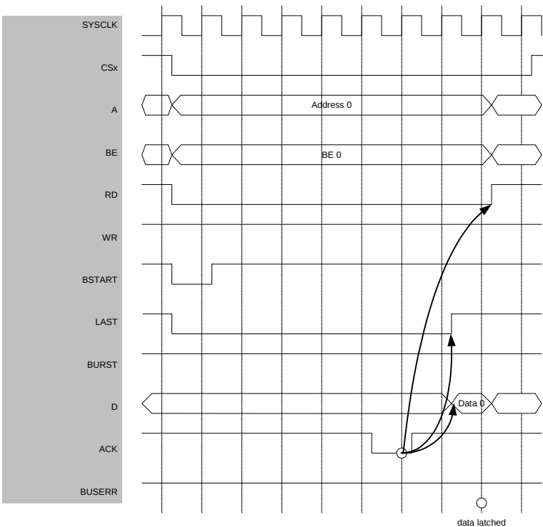
Figure 2.6.4 Waveform for External Acknowledge Mode Read Access Timing
