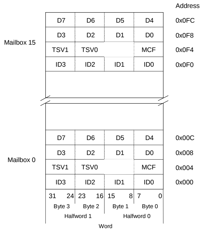
Figure 7.2.1 Mailbox RAM Structure
