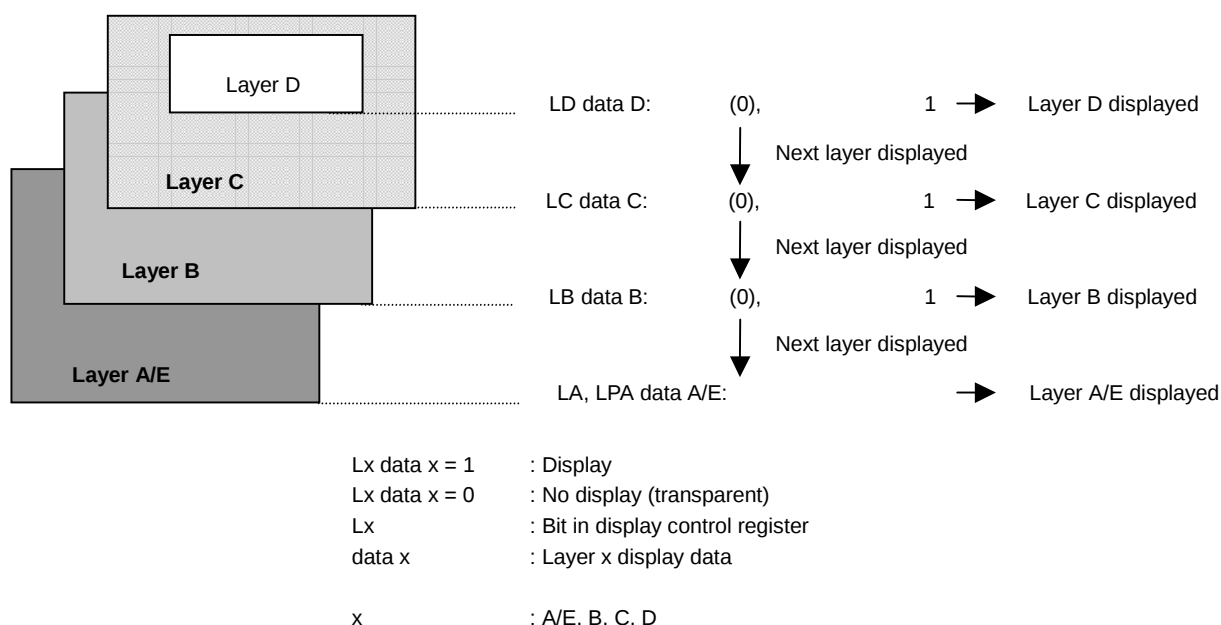
Figure 3.1.1 Layer Arrangement
