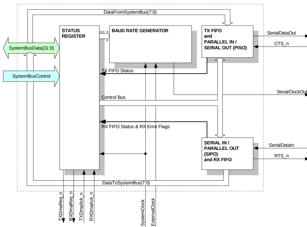
Figure 10.1.1 UART Block Diagram
