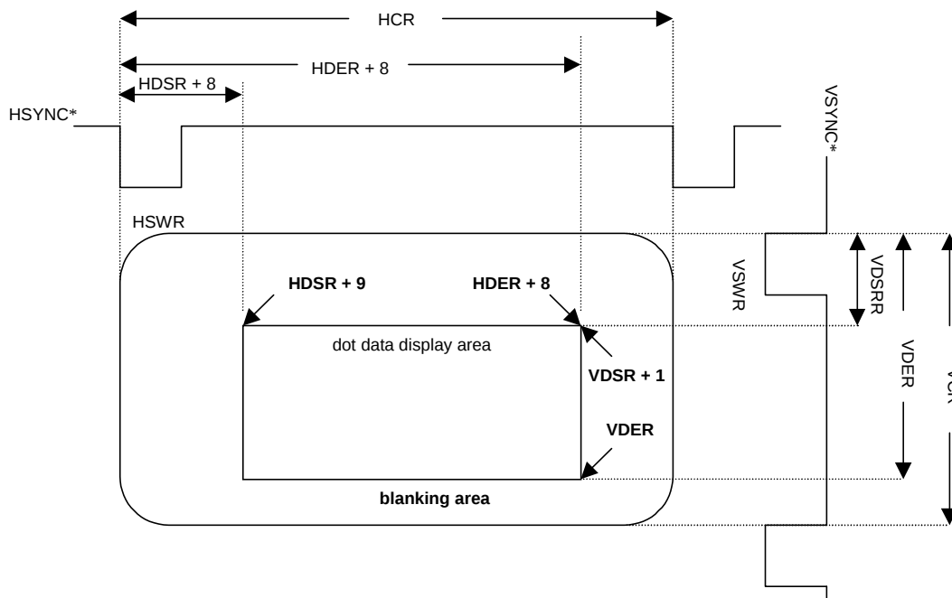
Figure 3.1.6 Display Timing
