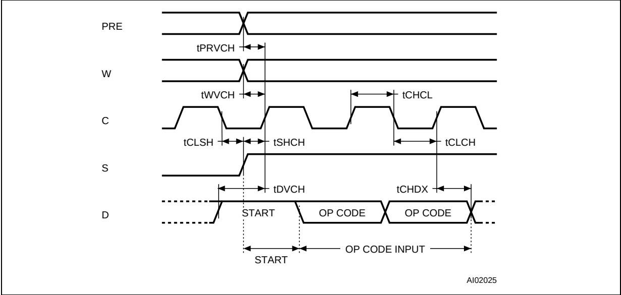
Figure 10. Synchronous Timing (Start and Op-Code Input)
