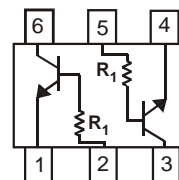
Device Schematic
