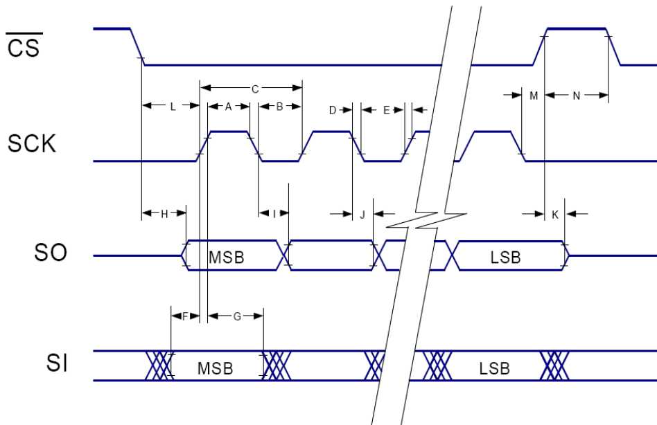
Figure 8. SPI Timing
