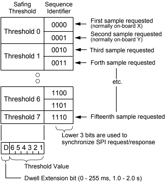
Figure 57. Safing Threshold Storage
