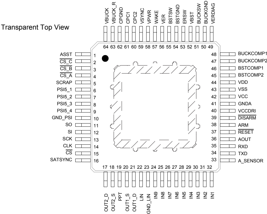
Figure 3. 33789 Pin Connections
