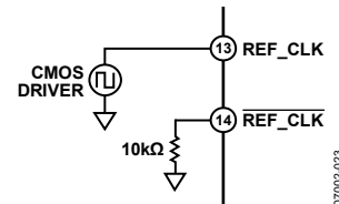
Figure 29. CMOS-Driven Diagram
