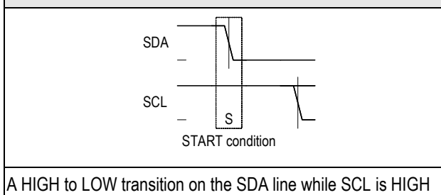
I 2 C Transmission Start Condition
