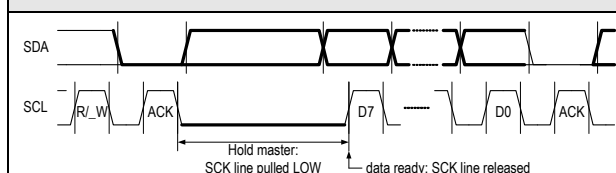
I 2 C Hold Master
