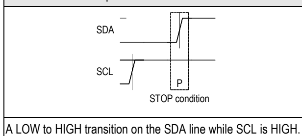
I 2 C Transmission Stop Condition
