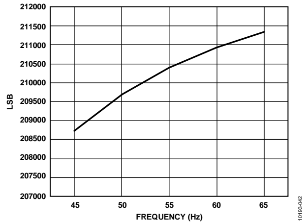
Figure 67. xIMAV Register Values at Full Scale, 45 Hz to 65 Hz Line Frequencies
