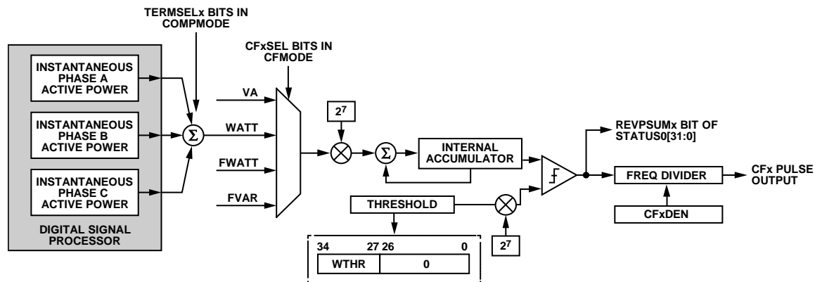
Figure 87. Energy-to-Frequency Conversion
