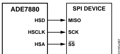
Figure 107. Connecting the ADE7880 HSDC with an SPI
