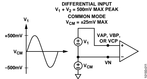
Figure 37. PGA in Current and Voltage Channels
