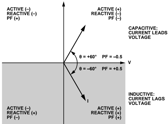
Figure 81. Capacitive and Inductive Loads
