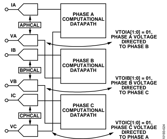
Figure 49. Phase Voltages Used in Different Datapaths
