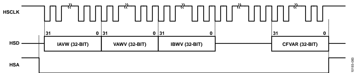
Figure 108. HSDC Communication for HGAP = 0, HXFER[1:0] = 00, and HSAPOL = 0; HSIZE is Irrelevant
