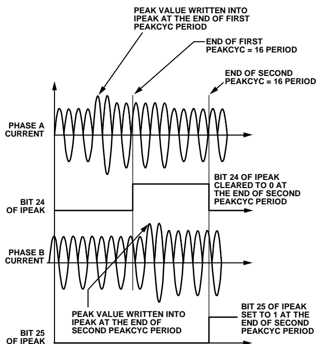
Figure 59. Peak Level Detection
