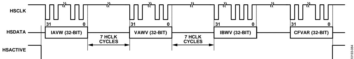
Figure 109. HSDC Communication for HSIZE = 0, HGAP = 1, HXFER[1:0] = 00, and HSAPOL = 0
