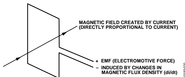
Figure 45. Principle of a di/dt Current Sensor
