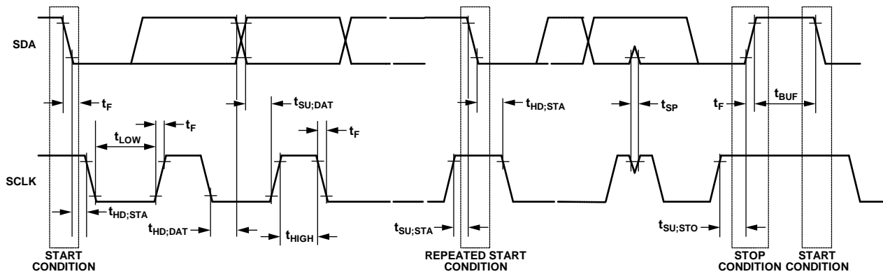
Figure 2. I²C-Compatible Interface Timing
