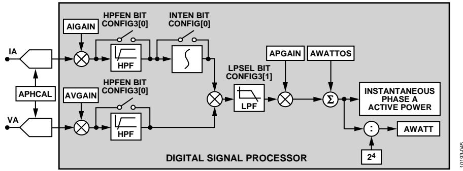
Figure 70. Total Active Power Data Path
