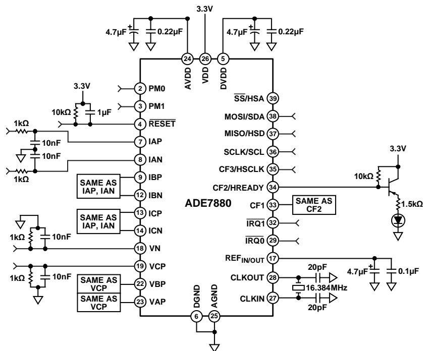
Figure 32. Test Circuit
