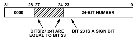
Figure 43. 24-Bit xIGAIN Transmitted as 32-Bit Words
