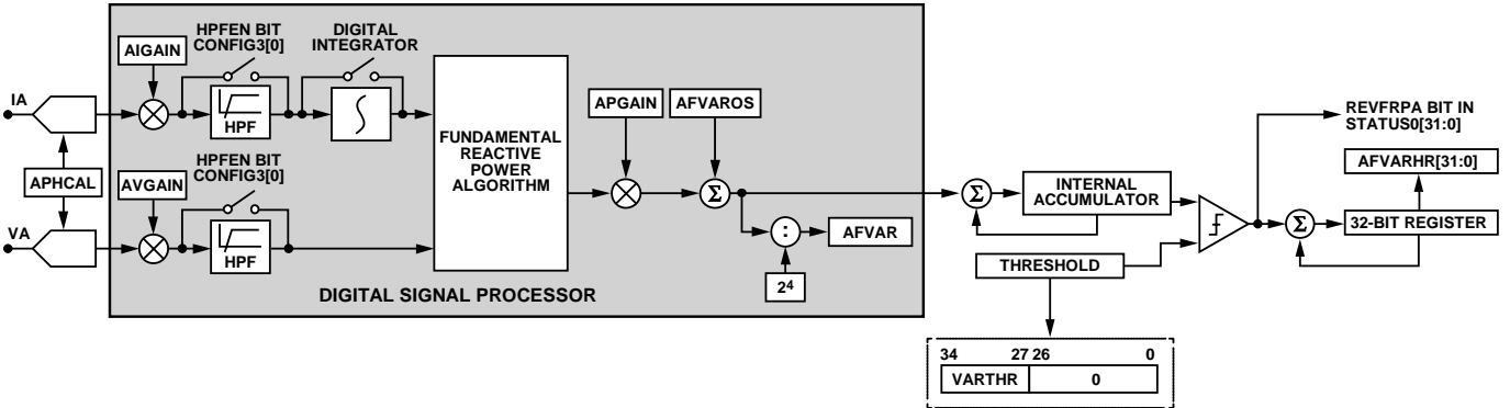
Figure 77. Fundamental Reactive Energy Accumulation
