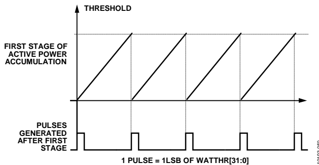
Figure 75. Active Power Accumulation Inside the DSP
