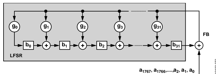
Figure 97. LFSR Generator Used in CHECKSUM Register Calculation
