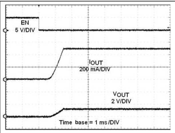
Figure 41. OC protection at V_{OUT} = 5.0\text{ V} (STMPS2161/2171- detail)
