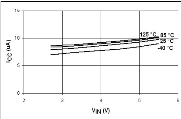
Figure 44. I_{CC} vs. V_{IN} (disabled) (STMPS2161/2171)
