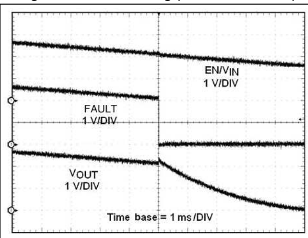
Figure 37. UVLO falling (STMP2161/2171)
