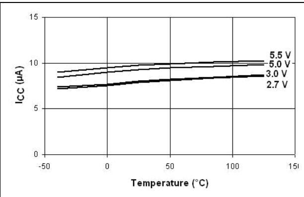
Figure 45. I_{CC} vs. temperature (disabled) (STMPS2161/2171)
