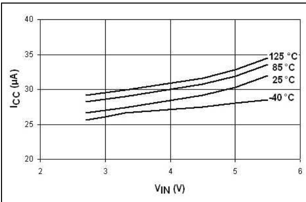
Figure 42. I_{CC} vs. V_{IN} (enabled) (STMPS2161/2171)
