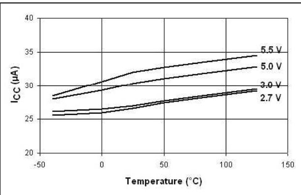
Figure 43. I_{CC} vs. temperature (enabled) (STMPS2161/2171)
