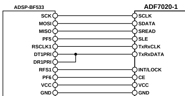
Figure 37. ADSP-BF533 to ADF7020-1 Connection Diagram
