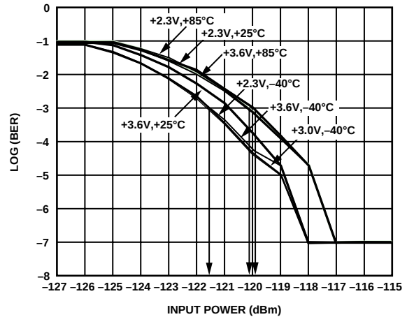
Figure 16. Sensitivity vs. V_{DD} and Temperature, RF = 315\text{ MHz} , DR = 1\text{ kbps} , Correlator Demod
