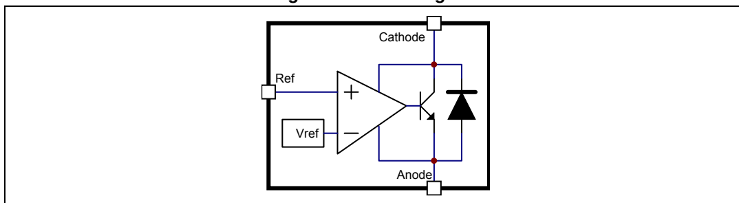
Figure 5. Block diagram
