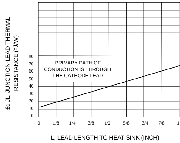
Fig. 10-TYPICAL THERMAL RESISTANCE
