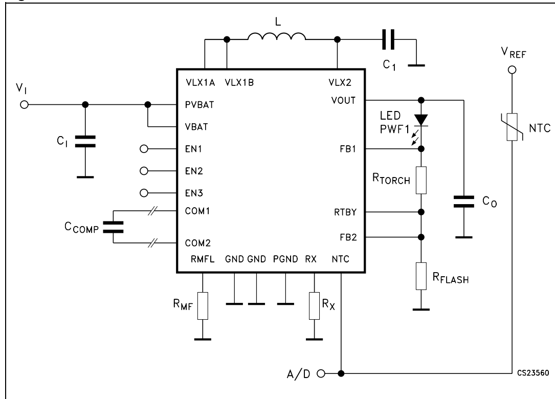
Figure 1. Schematic
