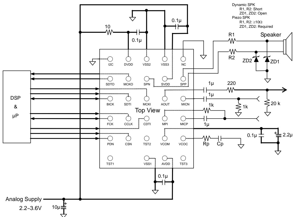
Figure 58. Typical Connection Diagram
