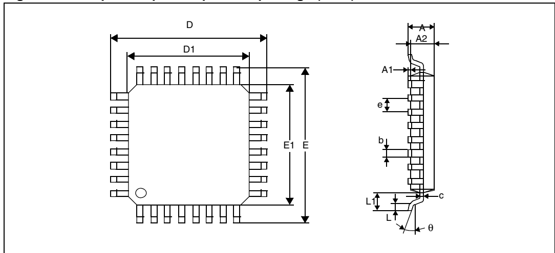
Figure 48. 32-pin low profile quad flat package (7 x 7)
