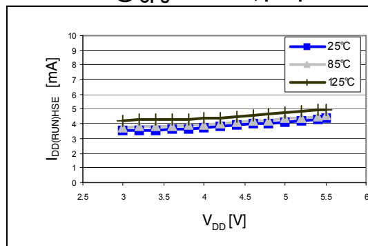
Figure 13. Typ. I_{DD(RUN)HSE} vs. V_{DD} @ f_{CPU} = 16 MHz, periph = on
