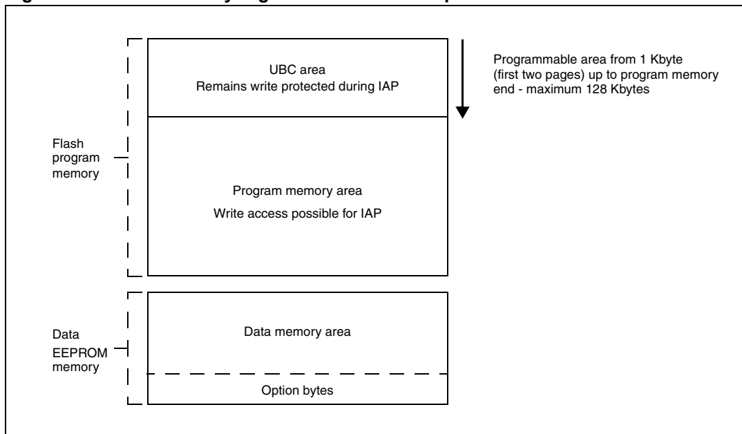
Figure 2. Flash memory organization of STM8A products
