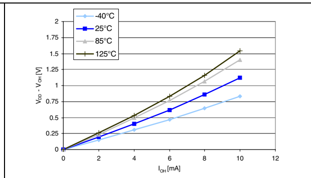
Figure 33. Typ. V_{DD} - V_{OH} @ V_{DD} = 5.0 V (standard ports)
