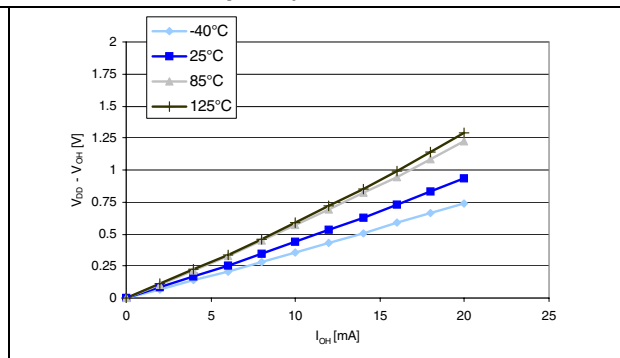
Figure 35. Typ. V_{DD} - V_{OH} @ V_{DD} = 5.0 V (high sink ports)
