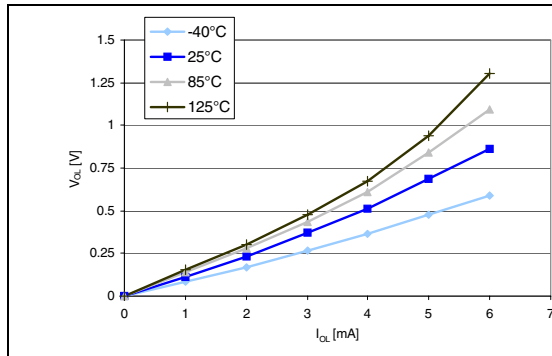
Figure 26. Typ. V_{OL} @ V_{DD} = 3.3 V (standard ports)
