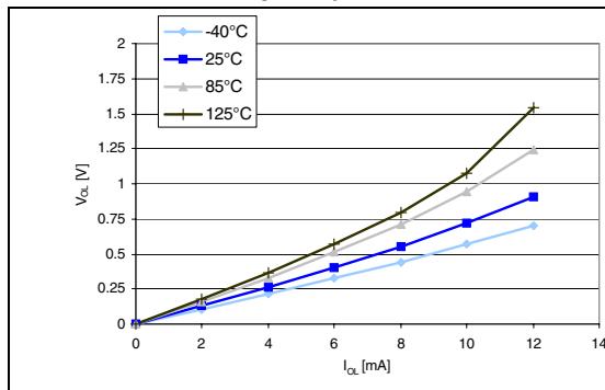
Figure 30. Typ. V_{OL} @ V_{DD} = 3.3 V (high sink ports)
