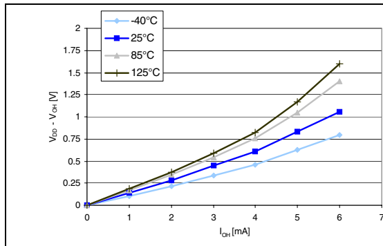
Figure 32. Typ. V_{DD} - V_{OH} @ V_{DD} = 3.3 V (standard ports)
