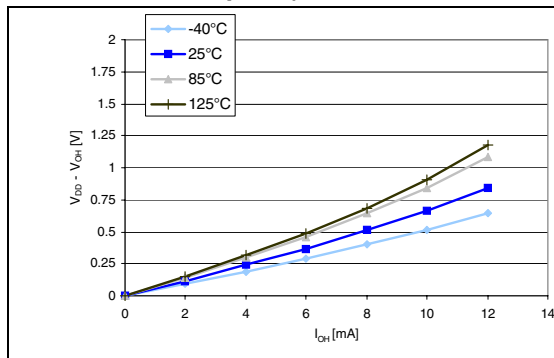
Figure 34. Typ. V_{DD} - V_{OH} @ V_{DD} = 3.3 V (high sink ports)
