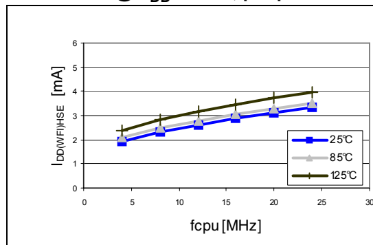
Figure 17. Typ. I_{DD(WFI)HSE} vs. f_{CPU} @ V_{DD} = 5.0 V, periph = on
