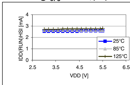
Figure 15. Typ. I_{DD(RUN)HSI} vs. V_{DD} @ f_{CPU} = 16 MHz, periph = off
