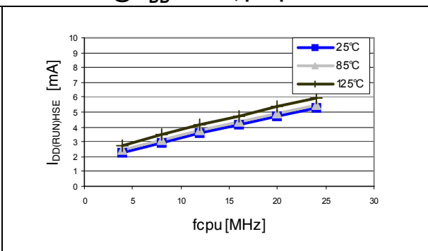
Figure 14. Typ. I_{DD(RUN)HSE} vs. f_{CPU} @ V_{DD} = 5.0 V, periph = on
