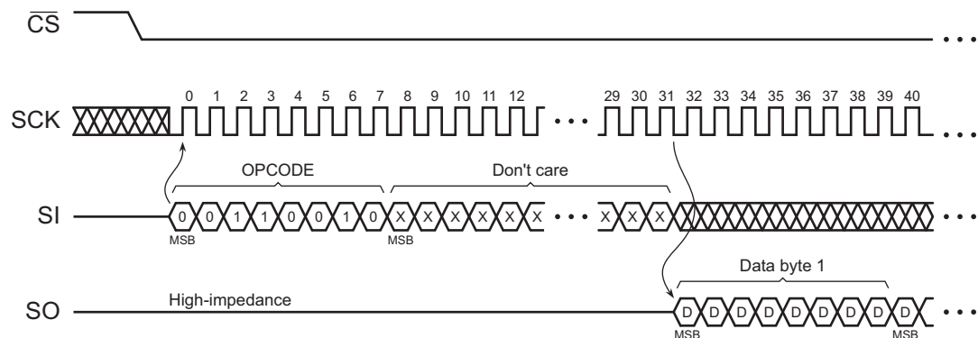
Figure 22-7. Read Sector Protection Register (Opcode 32H)
