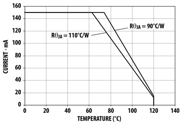
Figure 6a. Maximum Forward Current Vs. Ambient Temperature. Derated Based on T_{JMAX} = 125^{\circ}\text{C} , R_{\theta JA} = 110^{\circ}\text{C/W} & 90^{\circ}\text{C/W} .
