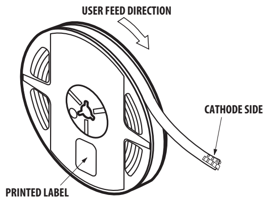
Figure 17. Reeling Orientation
