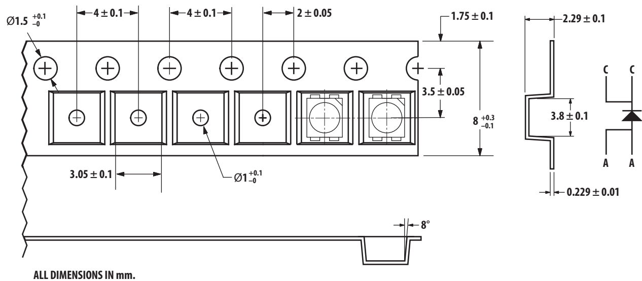
Figure 16. Tape Dimensions
