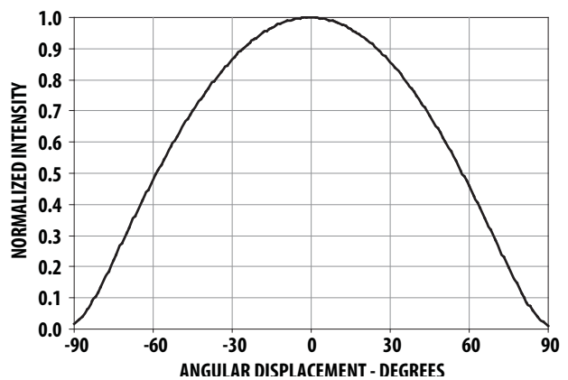
Figure 11. Radiation Pattern
