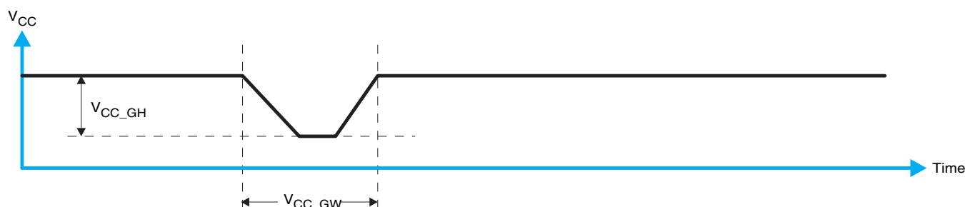
Figure 19. Glitch Width and Glitch Height
