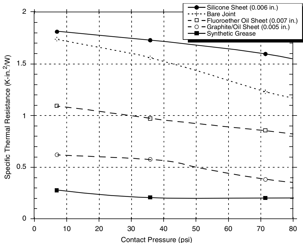
Figure 23. Thermal Performance of Select Thermal Interface Material
