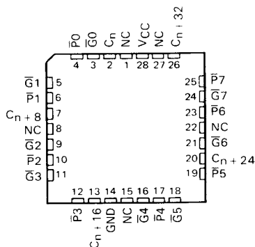
SN54AS882A ... FK PACKAGE SN74AS882A ... FN PACKAGE (TOP VIEW)
