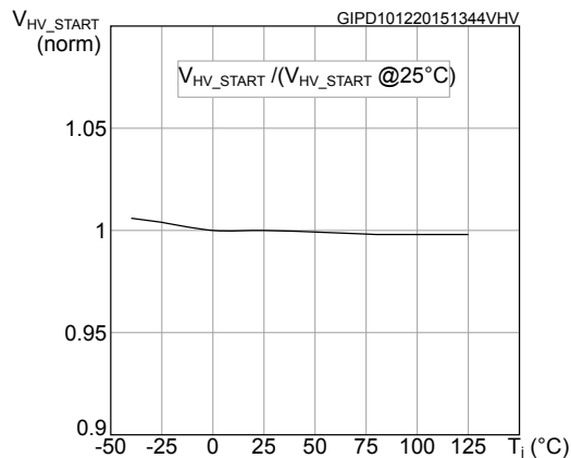
Figure 6. V_{HV\_START} vs T_J
